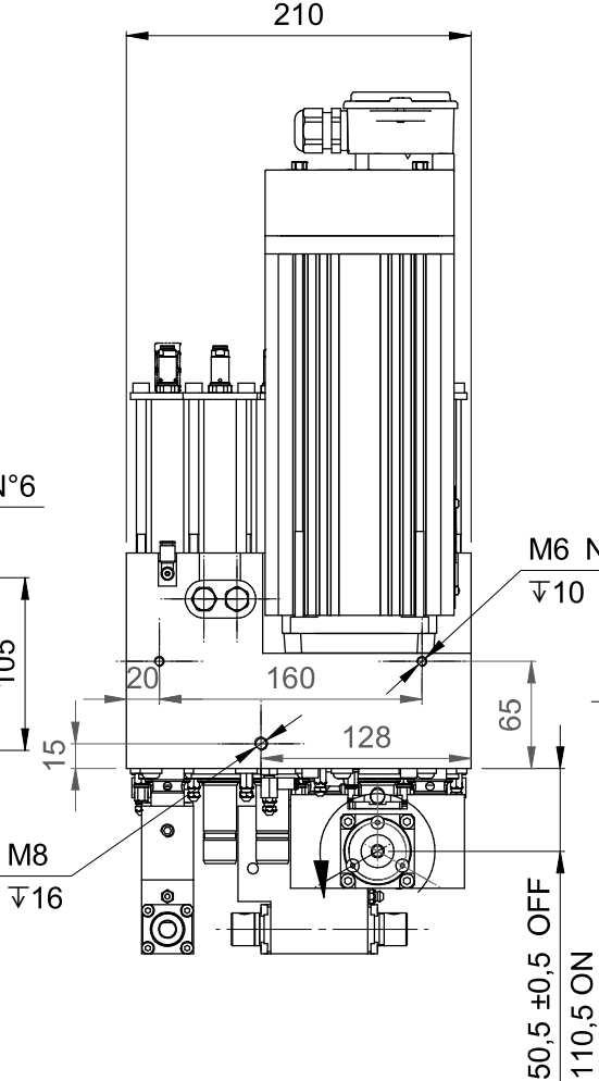
VERTICAL AND HORIZONTAL SPINDLE
