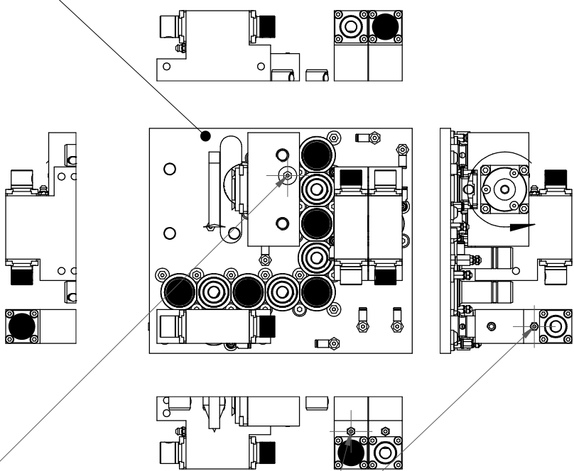
HORIZ. SPINDLES LUBRICATION POINTS
