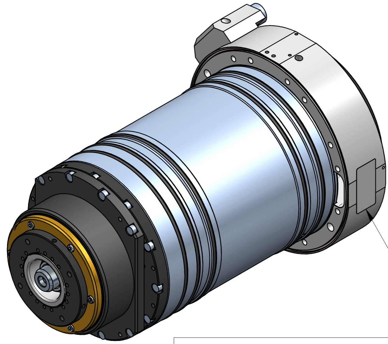
TARGHETTA IDENTIFICATIVA IDENTIFICATION PLATE Cod. 03L0441668H
